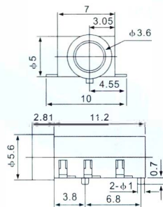
PJ-3013D
