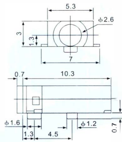
PJ-20500
